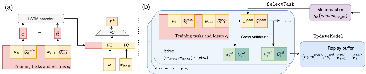
Figure 2: (a) the neural network architecture of the learning dynamics model with FCs representing the fully connected layers; (b) The meta-training pipeline of MM-ACL. More details of the pipeline are presented in Sec. 4.3
