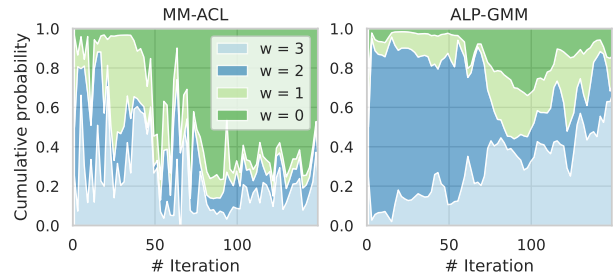
Figure 5: The probability distributions used by MM-ACL (left) and ALP-GMM (right) to sample source tasks at different training iterations in the same meta-testing lifetime.
