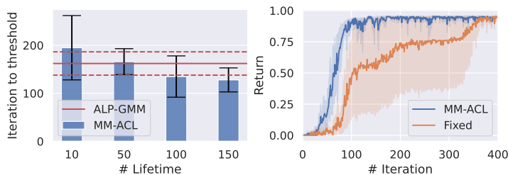
Figure 6: (left) the sample efficiencies of MM-ACL (blue) trained for 10, 50, 100, and 150 lifetimes, with the red solid line marking the sample efficiency of ALP-GMM, and the dashed lines marking its 95% confidence interval; (right) evaluation of the target task return of the students taught by MM-ACL and a fixed curriculum generated by MM-ACL.
